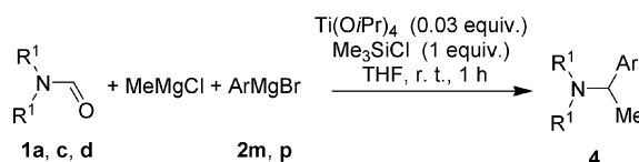
Scheme 2. Tertiary sec -alkylamines with two different substituents at the \alpha -carbon from N,N -dialkylformamides and two different Grignard reagents. For details see Table 2.
